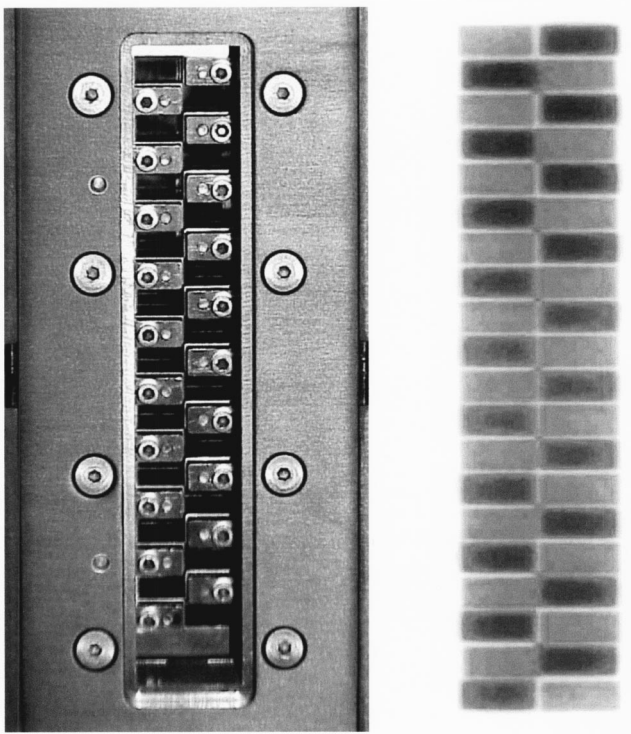
FIG. II.4. Checkerboard pattern design using MIMiC ® leaves and the resulting exposed film from laterals. Reprinted with permission from Saw et al. (Ref. 27).
