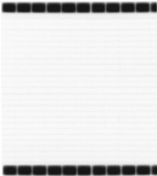
FIG. II.3. (a) MLC test pattern with all the leaves closed together except for the first and last pair, which have a 2 cm opening to force the upper jaws to remain open. (b) QA film produced by moving the pattern in 2 cm intervals and irradiating in a step-and-shoot fashion. Incomplete abutments will show as strips of increased density. This MLC has a focused leaf end design and abutting leaves should close completely.
