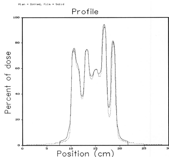
FIG. III.4. The dose profile measured with film across one line of a random intensity pattern (plan=dotted, film=solid), showing some systematic differences in low intensity regions.
