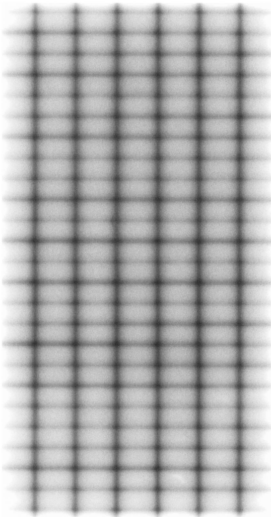
FIG. II.2. (a) MLC test pattern with a 1 mm wide strip. (b) QA film produced by moving the pattern in 2 cm intervals and irradiating in a step-and-shoot fashion. This MLC has a rounded leaf end design.
