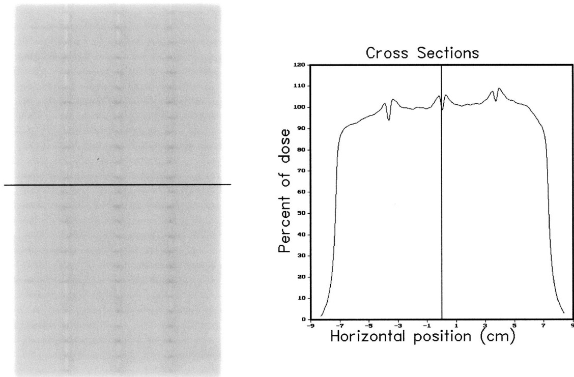
FIG. II.1. (a) MLC test pattern with a 2 cm wide strip. (b) QA film produced by moving the pattern in 2 cm intervals and irradiating in a step-and-shoot fashion. The strips should abut at the 50% decrement lines as described in Sec. II A 1. The line on the film shows the location of the scan (c), which is used to assess the quality of the matching. This MLC has a rounded leaf end design.
