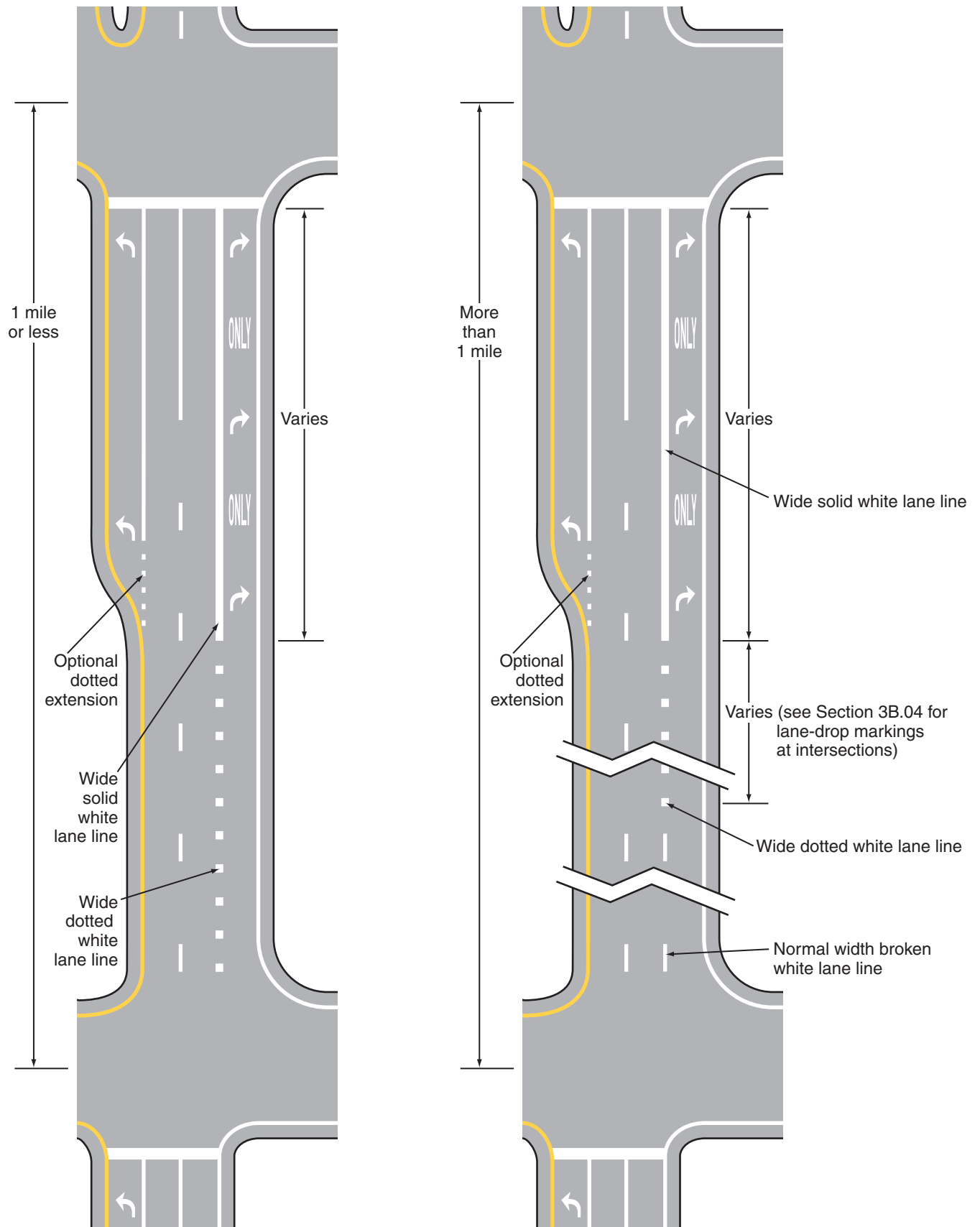
Figure 3B-11. Examples of Applications of Conventional Road Lane-Drop Markings (Sheet 2 of 2)
