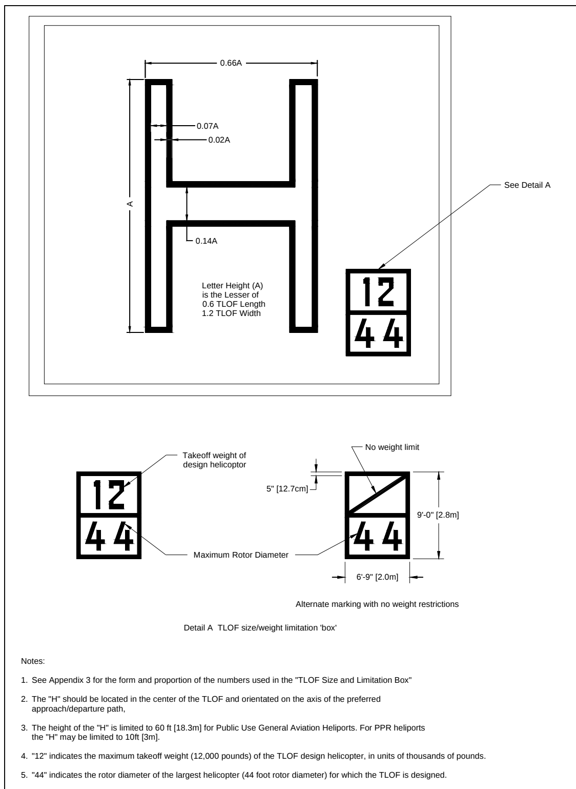
Figure 2-22. Standard Heliport Identification Symbol, TLOF Size and Weight Limitations:
