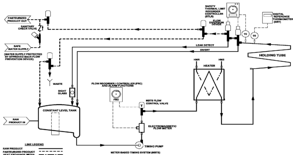
Figure 38. HTST Pasteurizer, without a Regenerator or Cooler Section, with a Meter Based Timing System Located Upstream from an Evaporator
