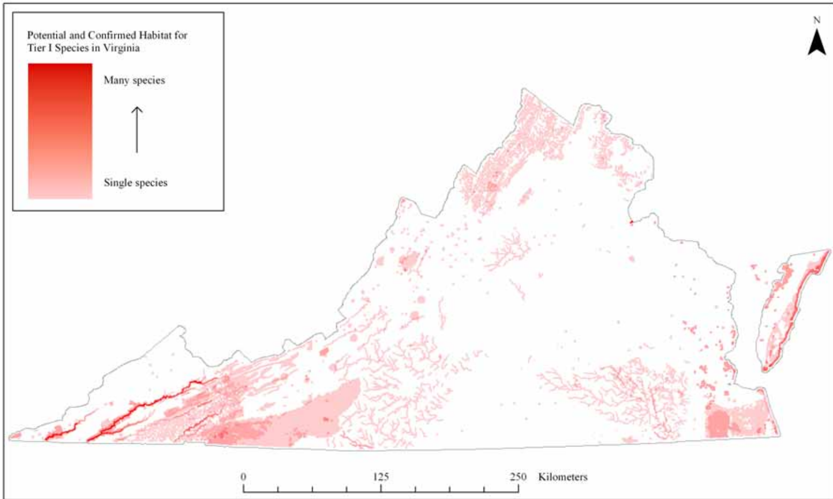
Figure 10.1. Potential and confirmed habitat for Tier I species. Darker shades represent areas with a higher co-occurrence of these habitats. See Chapters 4-9 for maps of individual species and compilations within each ecoregion.
