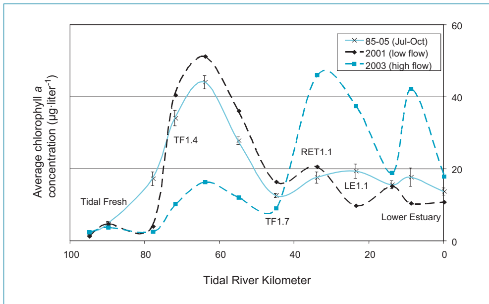
Figure IV-4. Average surface chlorophyll a concentrations in the tidal Patuxent River during the late growing season (July–October from 1985–2005) by Chesapeake Bay Water Quality Monitoring Program station with high- and low-flow years. Standard error bars are shown for the long-term average.
