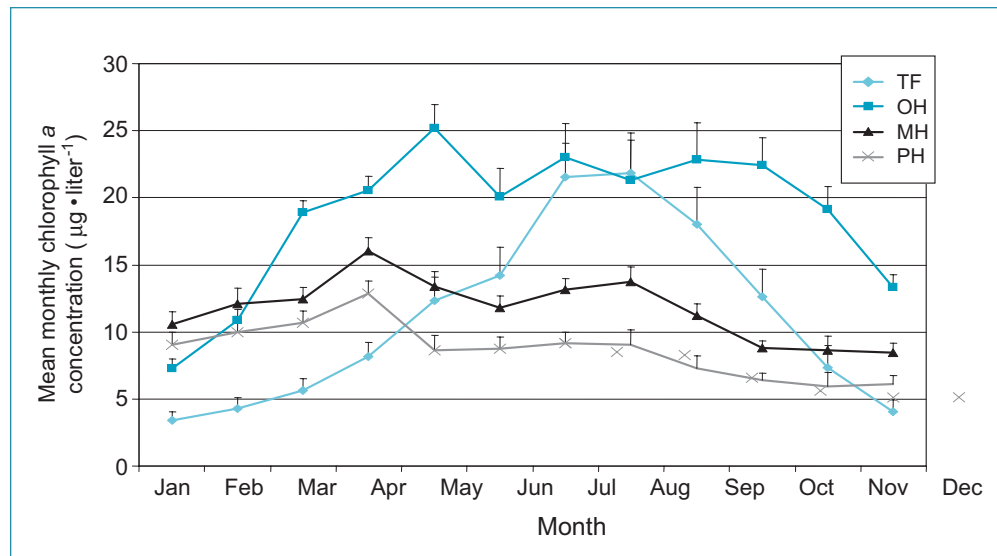
Figure IV-2. Mean monthly surface chlorophyll a concentrations for the tidal fresh (TF), oligohaline (OH), mesohaline (MH) and polyhaline (PH) salinity zones of the Chesapeake Bay (1985–2004) with standard error bars.
