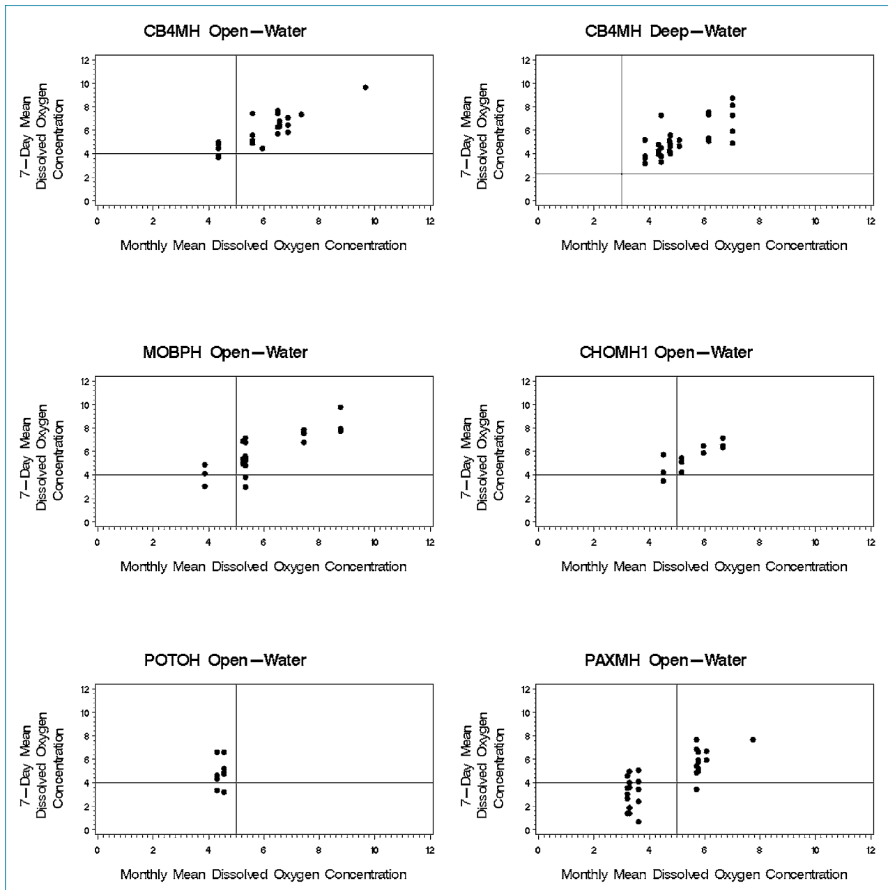
Figure V-4. Plots of monthly mean dissolved oxygen concentration (mg liter -1 ) versus the 7-day mean dissolved oxygen concentration (mg liter -1 ) in several example Chesapeake Bay Program segments: open-water and deep-water middle central Chesapeake Bay (CB4MH), Mobjack Bay (MOBPH), lower Choptank River (CHOMH1), middle Potomac River (POTOH) and lower Patuxent River (PAXMH).
