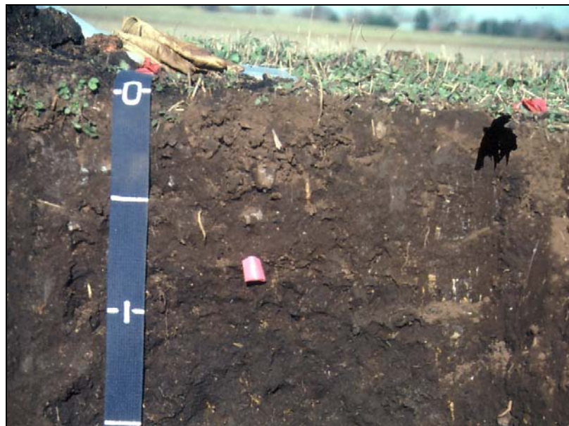
Figure 68. Black parent materials can mask redoximorphic features.
