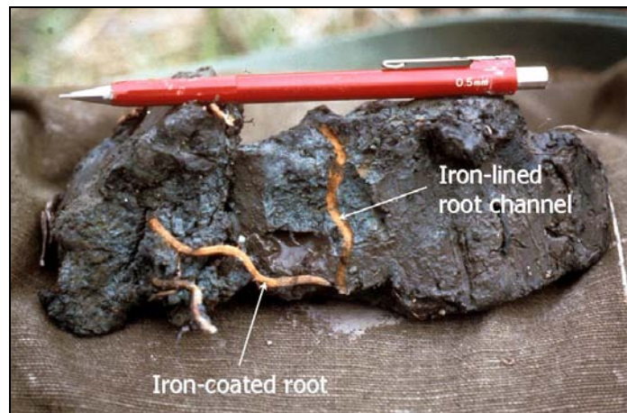
Figure 57. Iron-oxide plaque (orange coating) on a living root. Iron also coats the channel or pore from which the root was removed.
