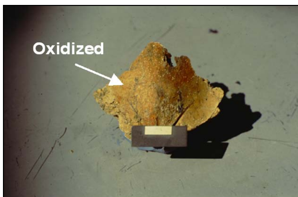
Figure 74. The same soil as in Figure 73 after exposure to the air and oxidation has occurred.
