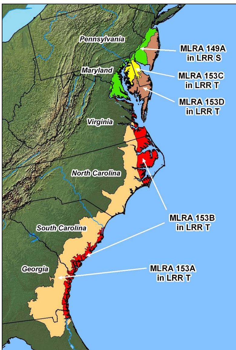
Figure 70. Locations of MLRAs 149A, 153A, 153B, 153C, and 153D.
