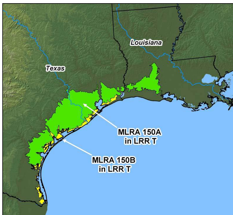
Figure 33. Location of MLRAs 150A and 150B.
