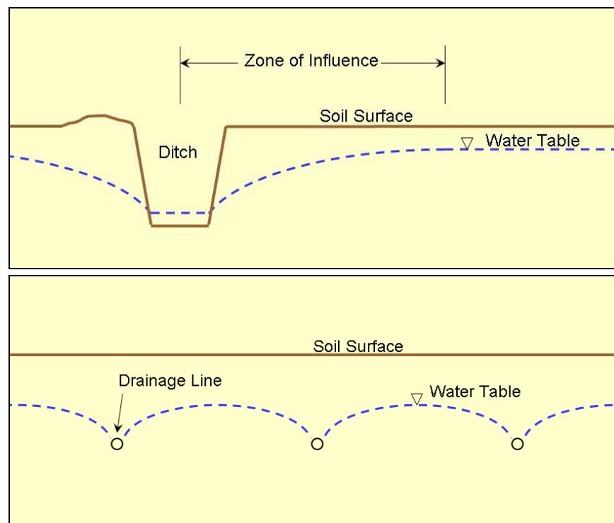
Figure 66. Effects of ditches (upper) and parallel subsurface drainage lines (lower) on the water table.
