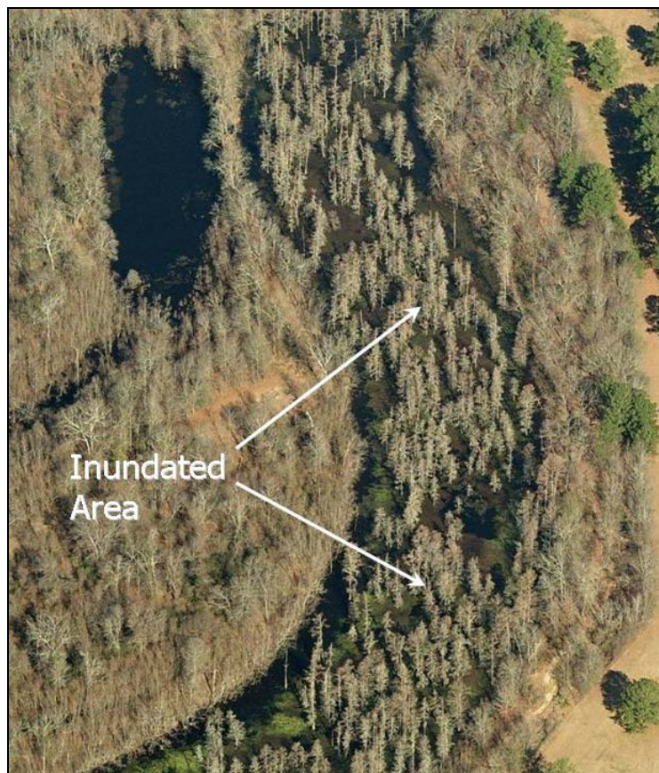
Figure 47. Aerial view of a forested wetland with surface water present.
