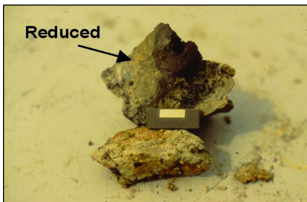
Figure 73. This soil exhibits colors associated with reducing conditions. Scale is 1 cm.
