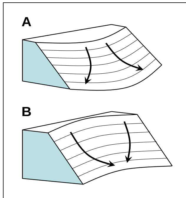
Figure 3. Divergent slopes (A) disperse surface water, whereas convergent slopes (B) concentrate water. Surface flow paths are indicated by the arrows.
